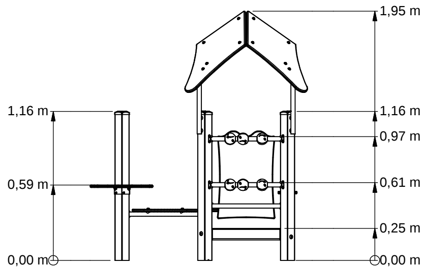
Achter (Back)
