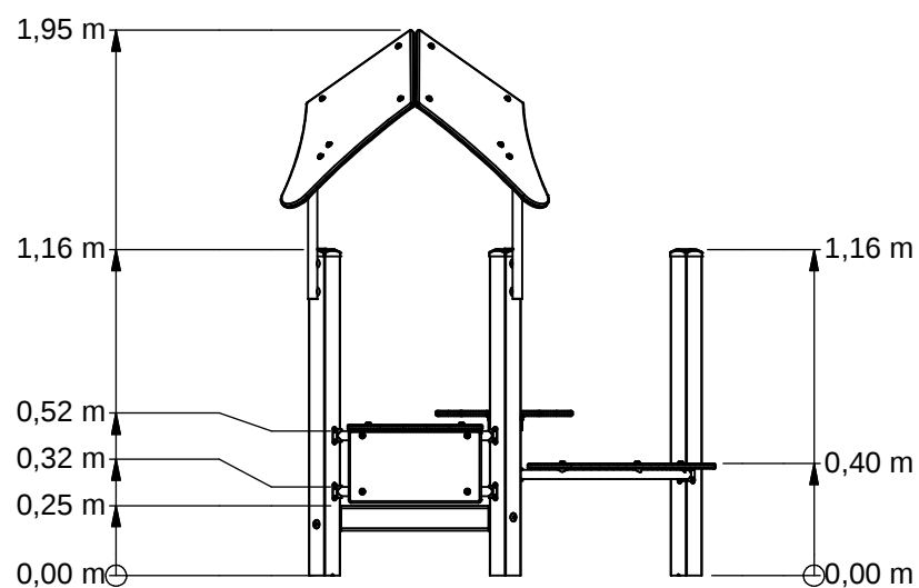
Links (Left)
