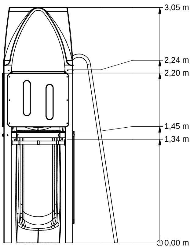
Achter (Back)
