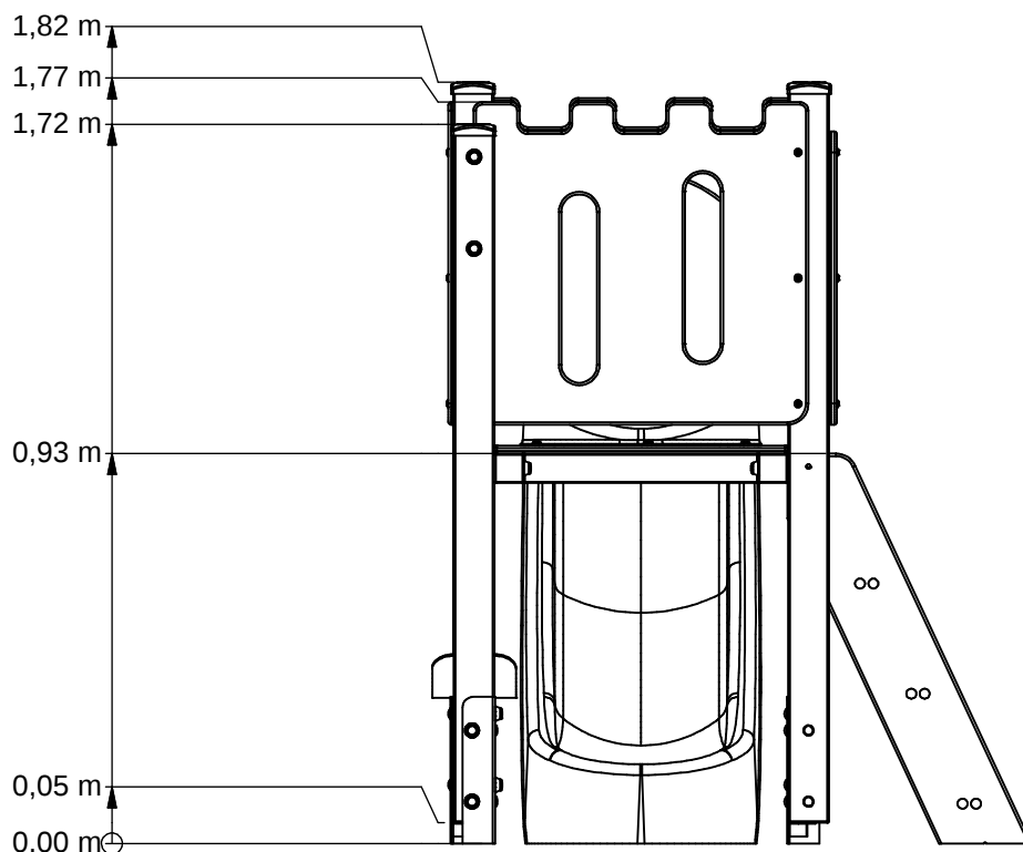
Achter (Back)
