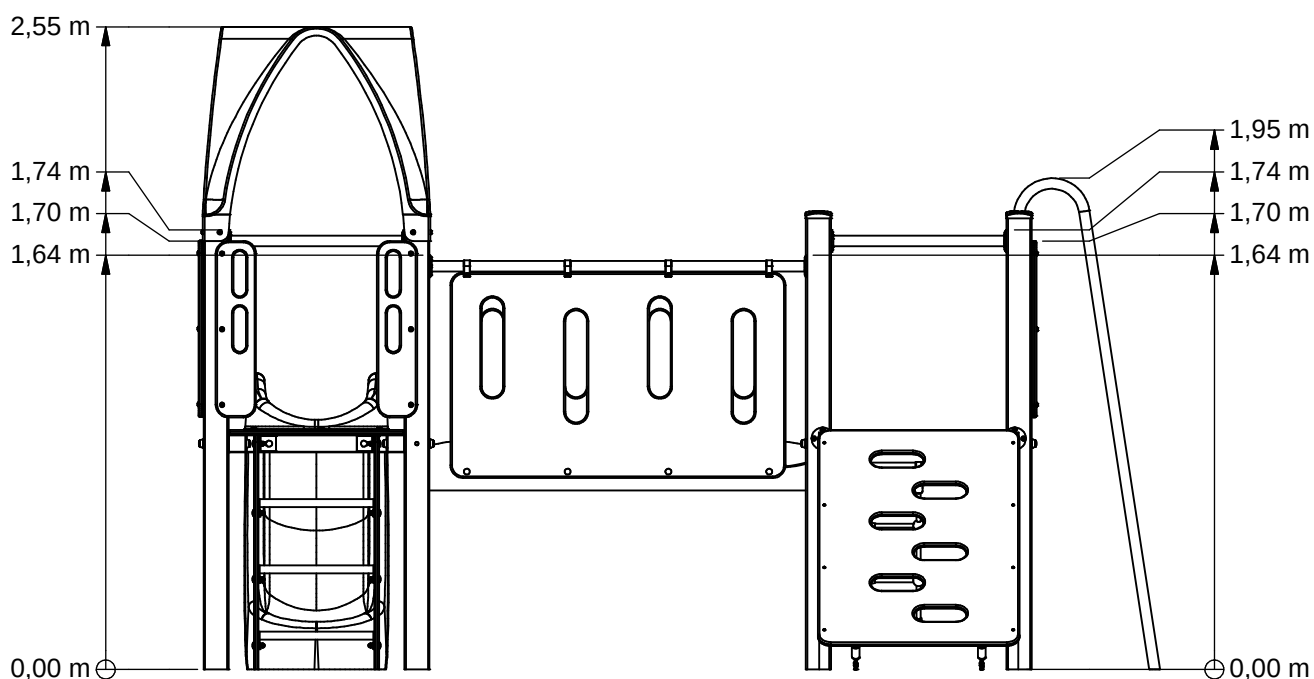
Achter (Back)
